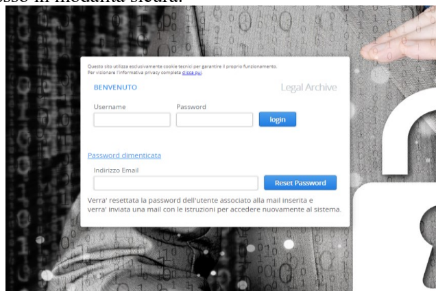
Figura 3 - Reset Password
